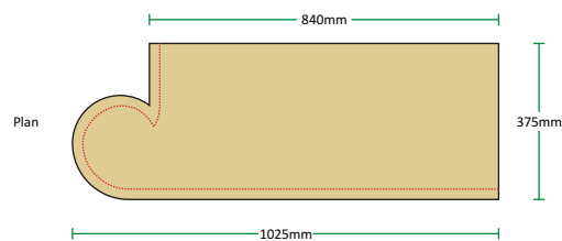
Curved Curtail Tread STC100-35 Available LH and RH
