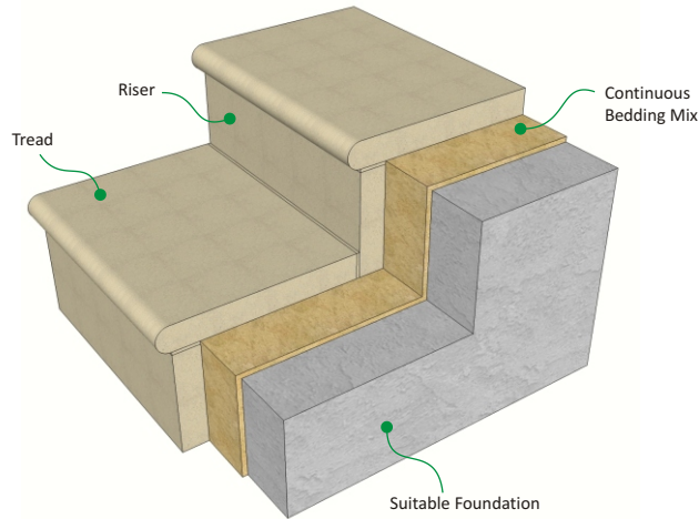
Return Tread STB available LH and RH (LH shown)
