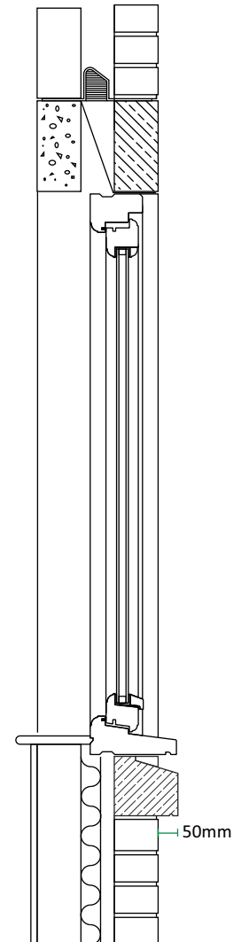
Section detail showing typical construction All joints shown 6mm
