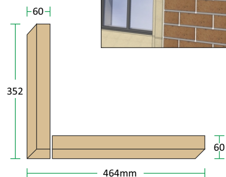
QC330 AND QC440 PLAN
