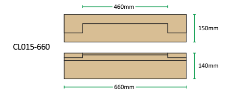
Plan and Elevation of our standard opening sizes
